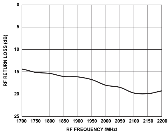
Figure 27. RF Port Return Loss, Fixed IF
