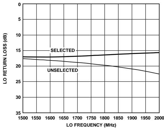
Figure 28. LO Return Loss, Selected and Unselected
